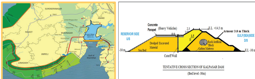
Figure 7 : Tentative layout and cross section of Kalpasar dam ( https://kalpasar.gujarat.gov.in/ )
