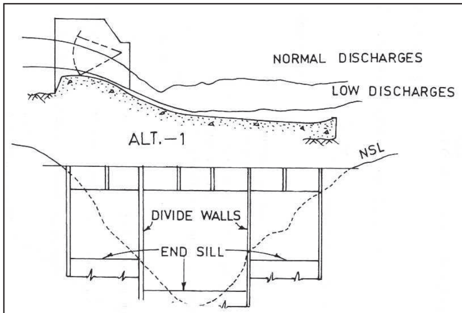
Figure 5 : Provision of spans at different levels (Khatsuria, 2004)
