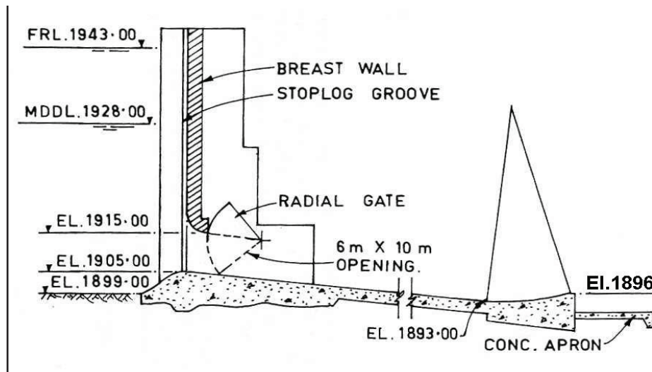
Figure 4 : Spillway cross section of Chukha dam spillway (Khatsuria, 2004)
