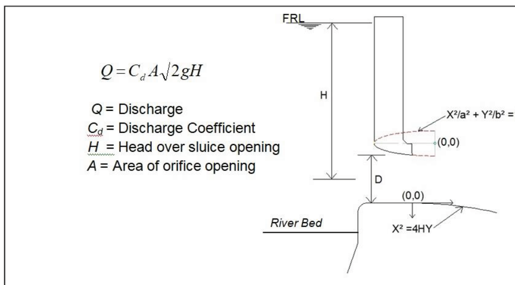
Figure 1 : Definition sketch of Orifice spillway
