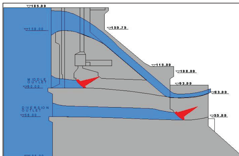
Figure 2 : Cross section of typical multi-level spillway
