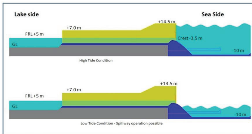
Figure 8 : The schematic view of the coastal reservoir spillway
