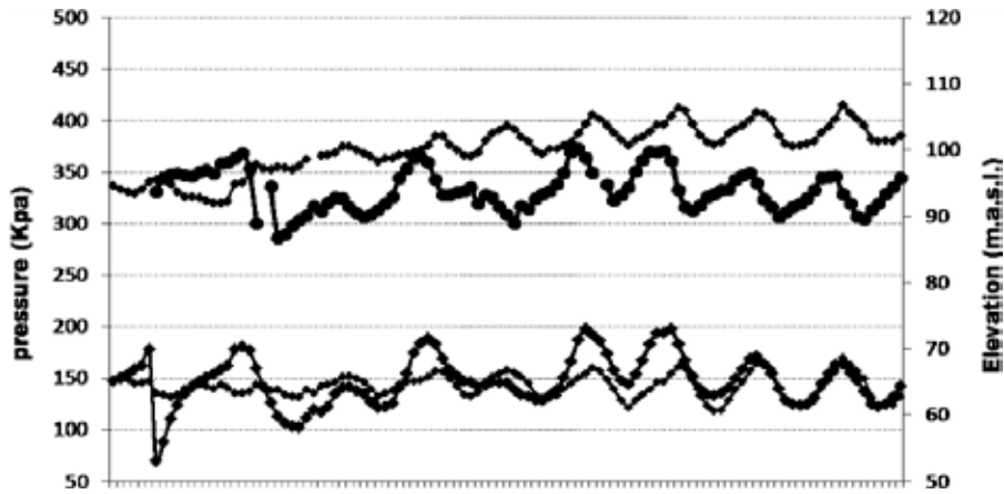
Figure 16 : Curves of reservoir water level fluctuations and vertical total pressure in section No.4
