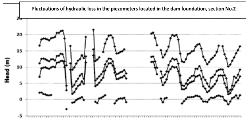
Figure 7 : The curves of hydraulic loss fluctuations per time in dam foundation section No.2
