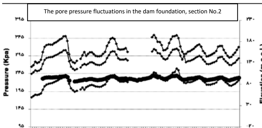
Figure 10 : The curves of pore pressure fluctuations in the dam foundation, section No.2
