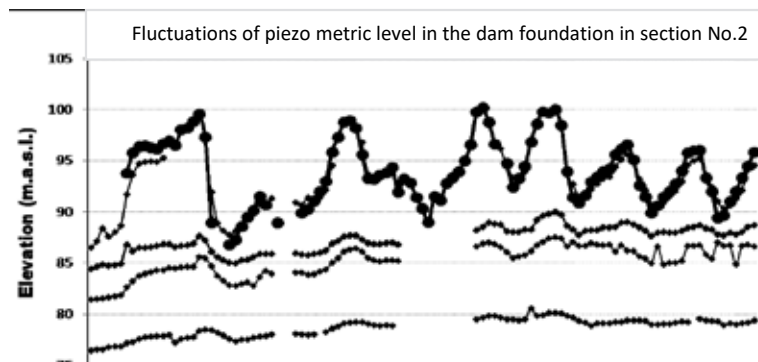
Figure 5 : The curves of piezometric level fluctuations over time in the dam foundation in section No.2
