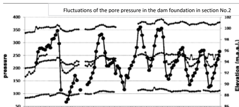
Figure 6 : The curves of the pore pressure fluctuations per time in the dam foundation section No.2
