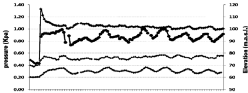
Figure 18 : Curves of the fluctuations of horizontal total pressure to vertical total pressure, and reservoir water level in section No.4
