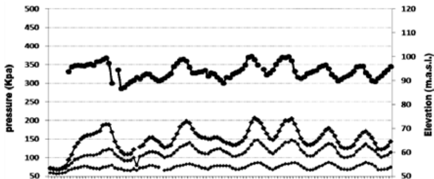
Figure 17 : Curves of reservoir water level fluctuations and horizontal total pressure in section No.4
