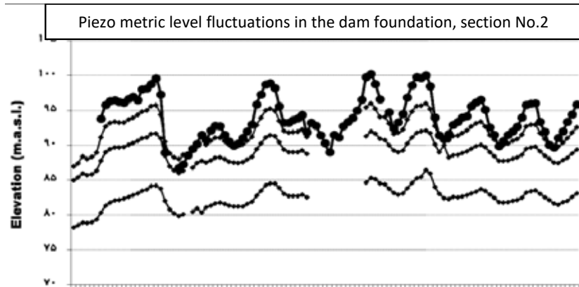
Figure 9 : Curves of piezometric level fluctuations per time in the dam foundation, section No.2
