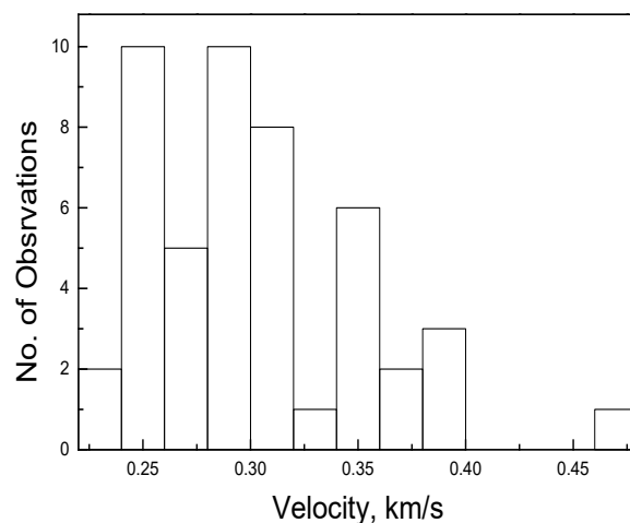
Figure 16 : P-wave velocities at Vihar dam near Durgah
