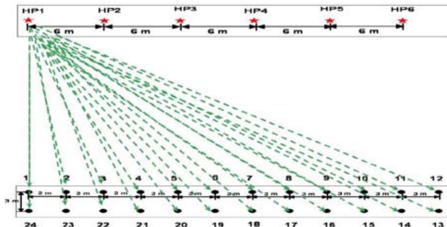
Figure 4 : Marking of geophones and location of Hammer points in Pattern – B for Masonry Dams
