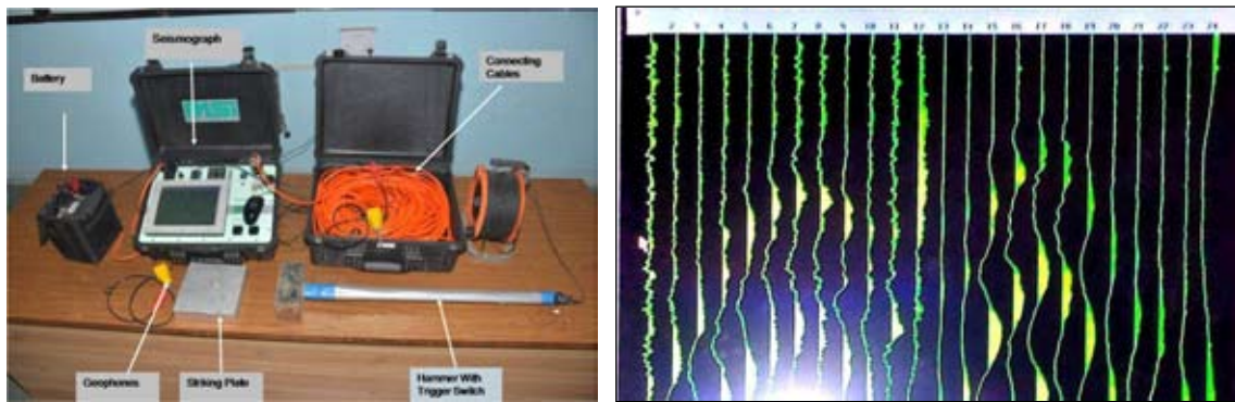
Figure 1 : 24-channel signal enhancement seismograph with accessories and a typical record showing the onset of P-waves at 24 locations
