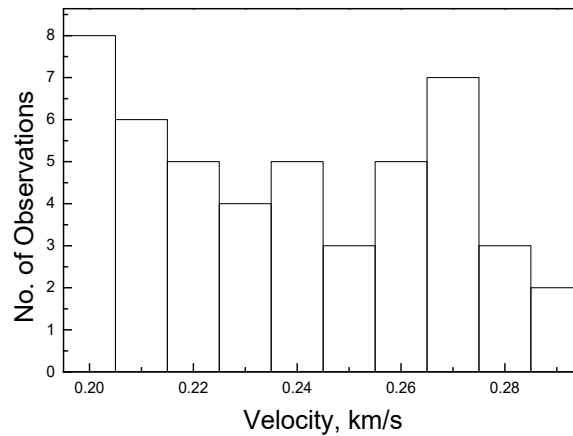
Figure 14 : P-wave velocities at Vihar dam near Durgah
