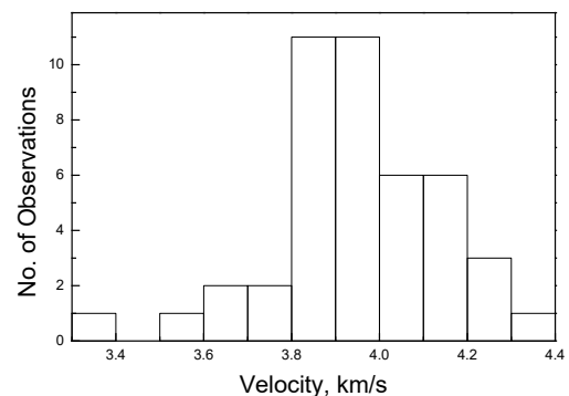
Figure 6 : P-wave velocities at Tulsi dam (Masonry)
