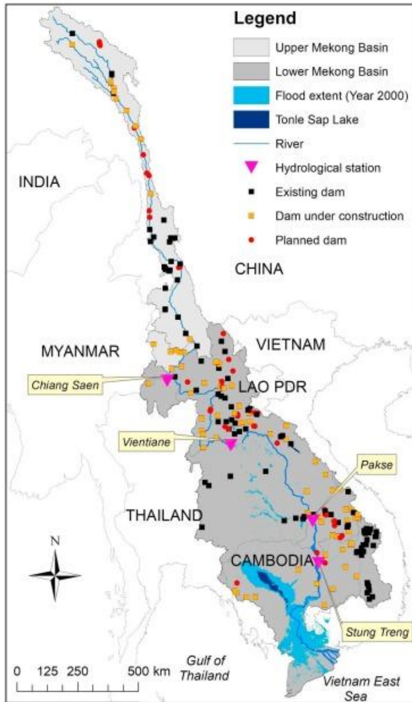
Figure2: Plan of dam cascades: Dams built or planned in the Mekong Basin along the Mekong River and tributaries (several dams along the upper and middle reaches of the Mekong are forming dam cascades, dam structures in middle and lower reaches form run-of-river power plant cascades)
