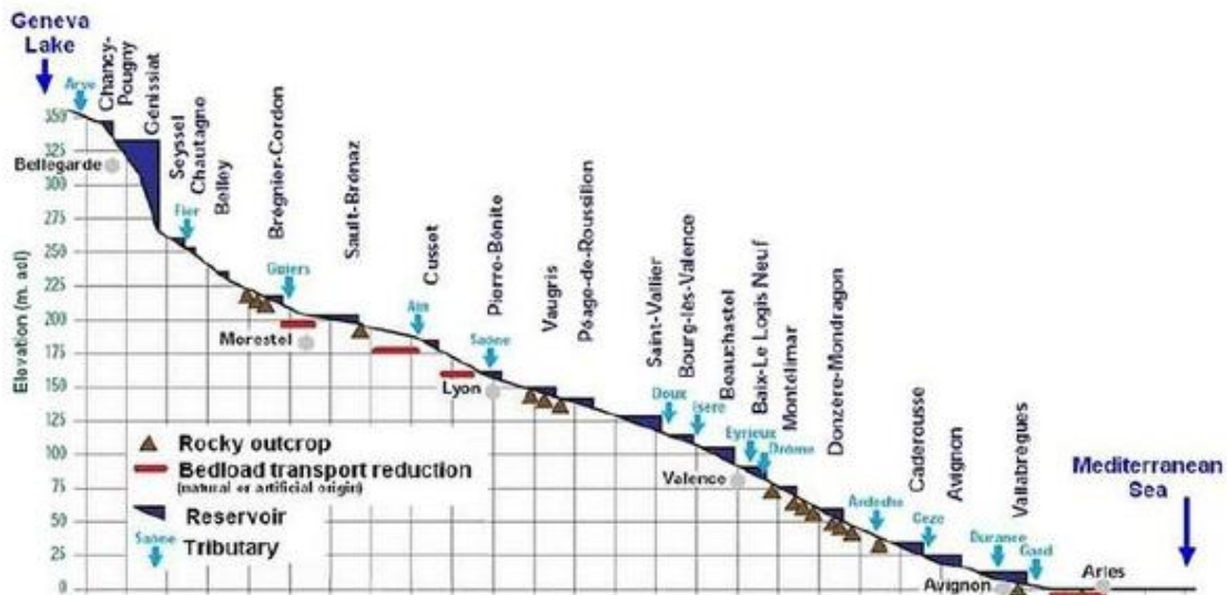
Figure 1: Longitudinal profile of the French Rhone River with cascade of run-of-river power plants (Peteuil2012)
