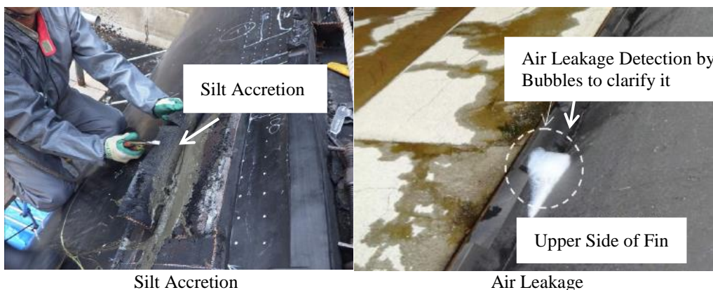
Figure 5. Representative damages nearfins
