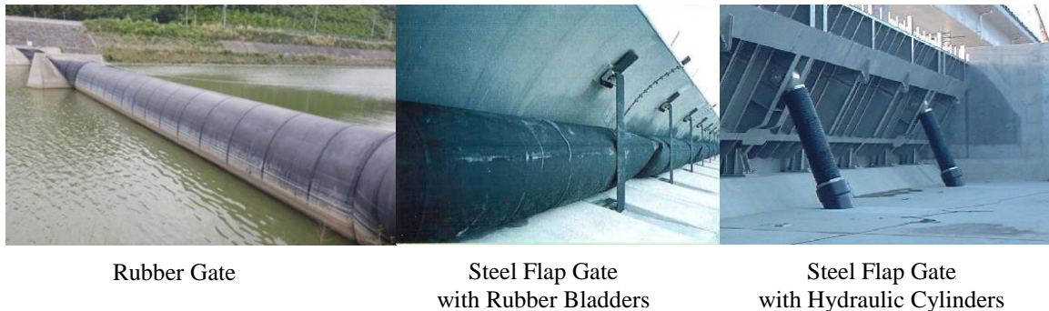
Figure 9. Samples of rubber gate and steel flap gate with rubber bladders and hydraulic cylinders
